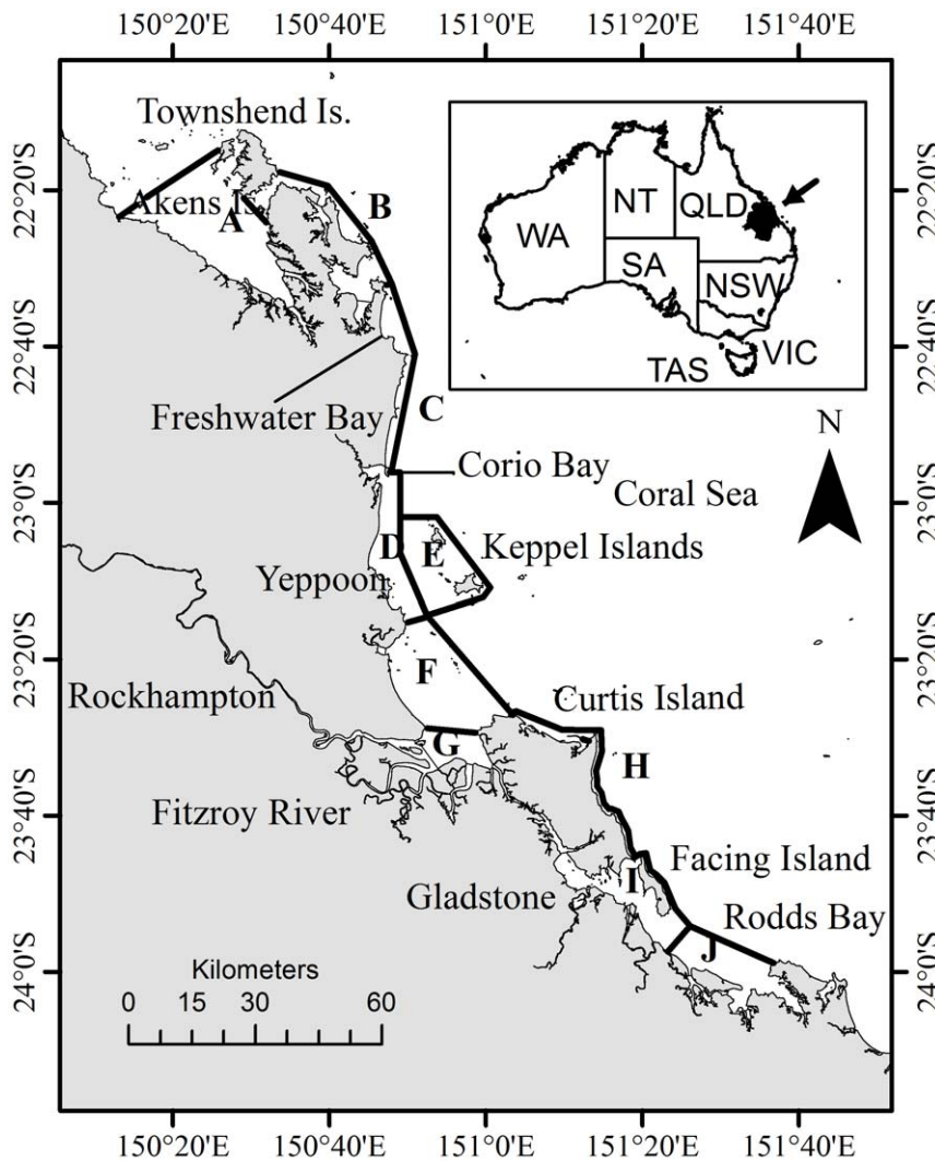
Figure 1. Map of the Capricorn Coast study area. Capital letters indicate survey sections: A=Shoalwater Bay, B=Northern Regions, C=Nine Miles Beach, D=Keppel Bay inshore, E=Keppel Islands, F=Fitzroy outer estuary, G=Fitzroy inner estuary and river, H=Curtis Island East Coast, I=North Port Curtis, J=South Port Curtis. Shoalwater Bay Military Training Area = A+B Keppel Bay = D+E+F+G, Port Curtis = I+J. doi:10.1371/journal.pone.0056729.g001
